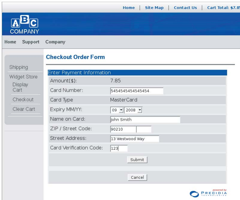
Figure 1. Checkout Screen
